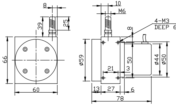
*DIMENSION (mm)
